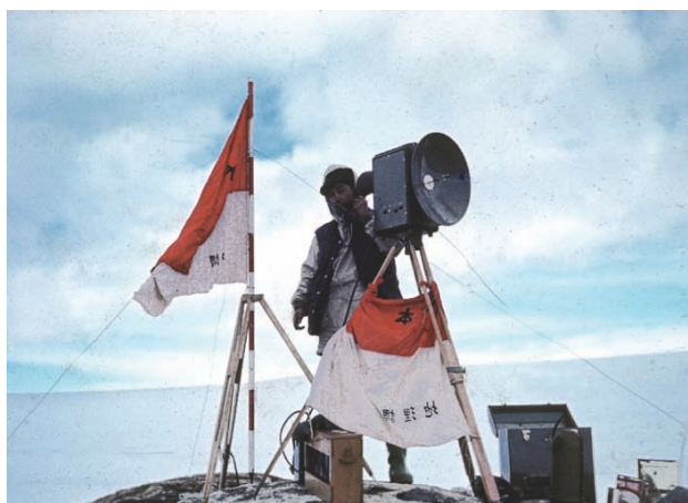
Photo 1 Observation by microwave distance meter, Tellurometer (JARE-4)
