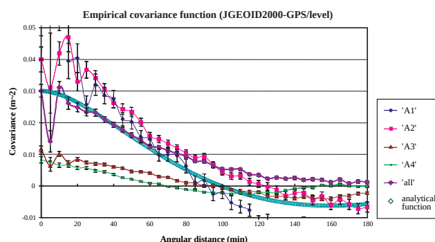
Fig. 6 Empirical and analytical covariance functions of geoid differences. A1 to A4 denote local areas.
