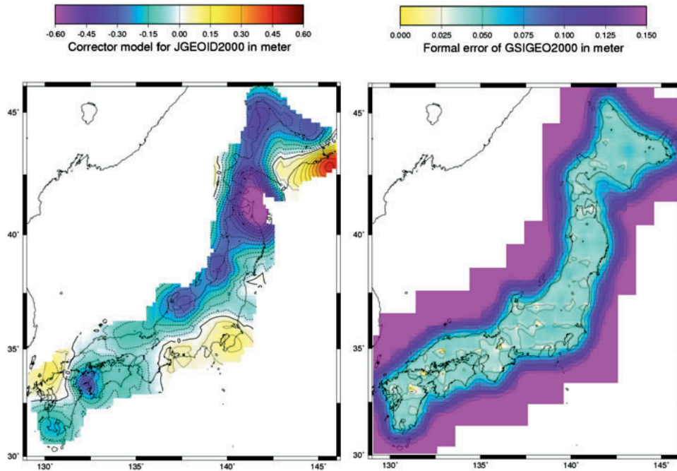
Fig. 7 Corrector model for gravimetric geoid (left) by least squares collocation and its formal error (right).
