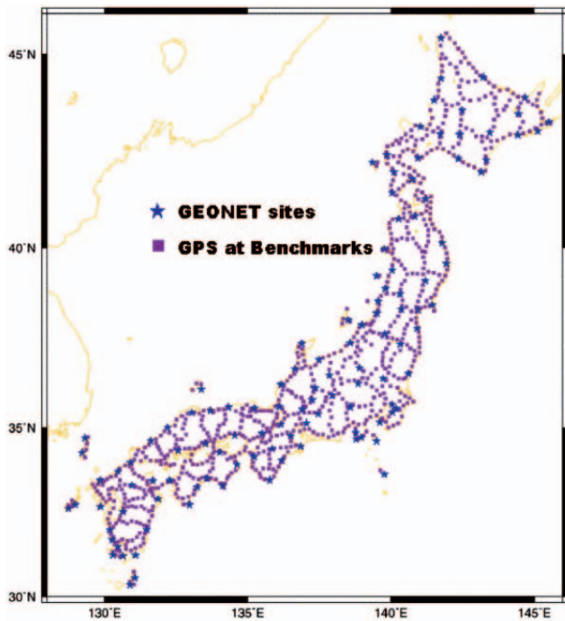
Fig. 2 Distribution of the nationwide net of GPS at benchmarks with GEONET sites.
