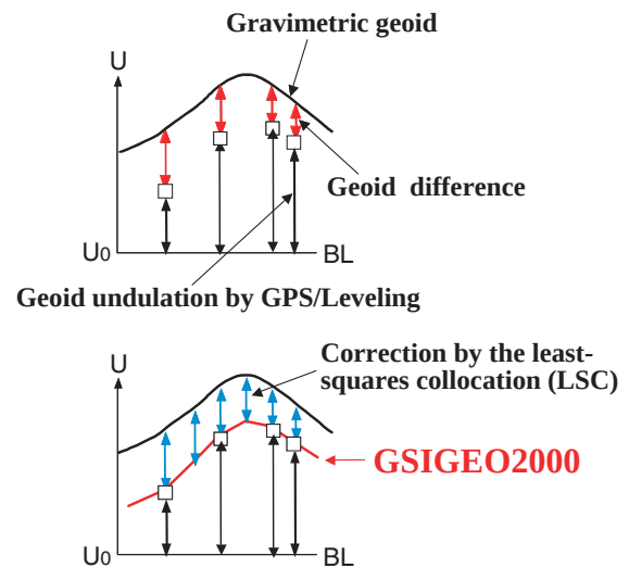
Fig. 4 Schematic diagram of hybrid geoid model construction.
