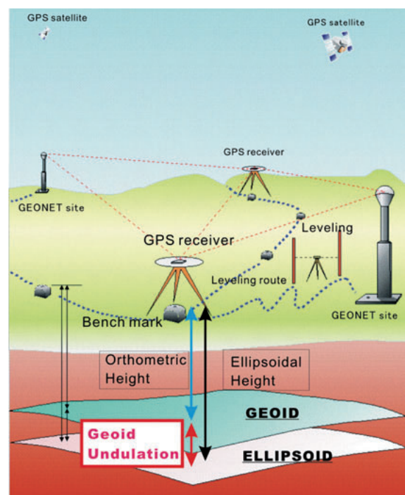
Fig. 1 Schematic figure of GPS/leveling survey.
