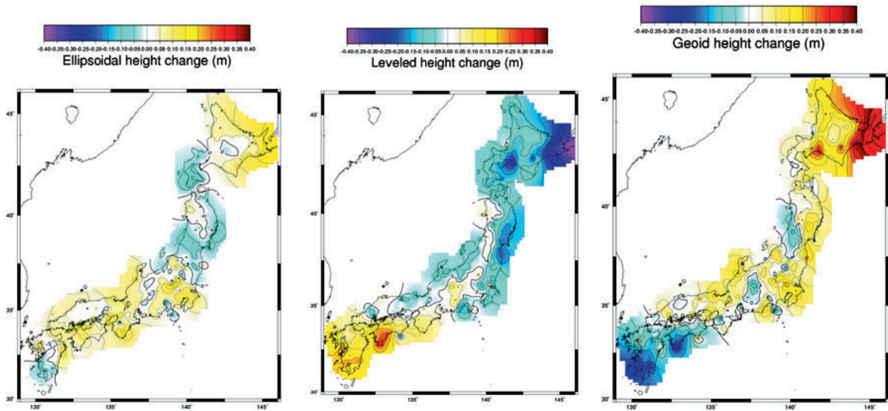
Fig. 3 The difference between the old and new analyses for GPS ellipsoidal heights (left), leveled heights (middle) and geoid undulation data (right). Color scale is -0.4\text{m} to 0.4\text{m} . Contour interval is 5\text{cm} and broken lines show contours of negative value.
