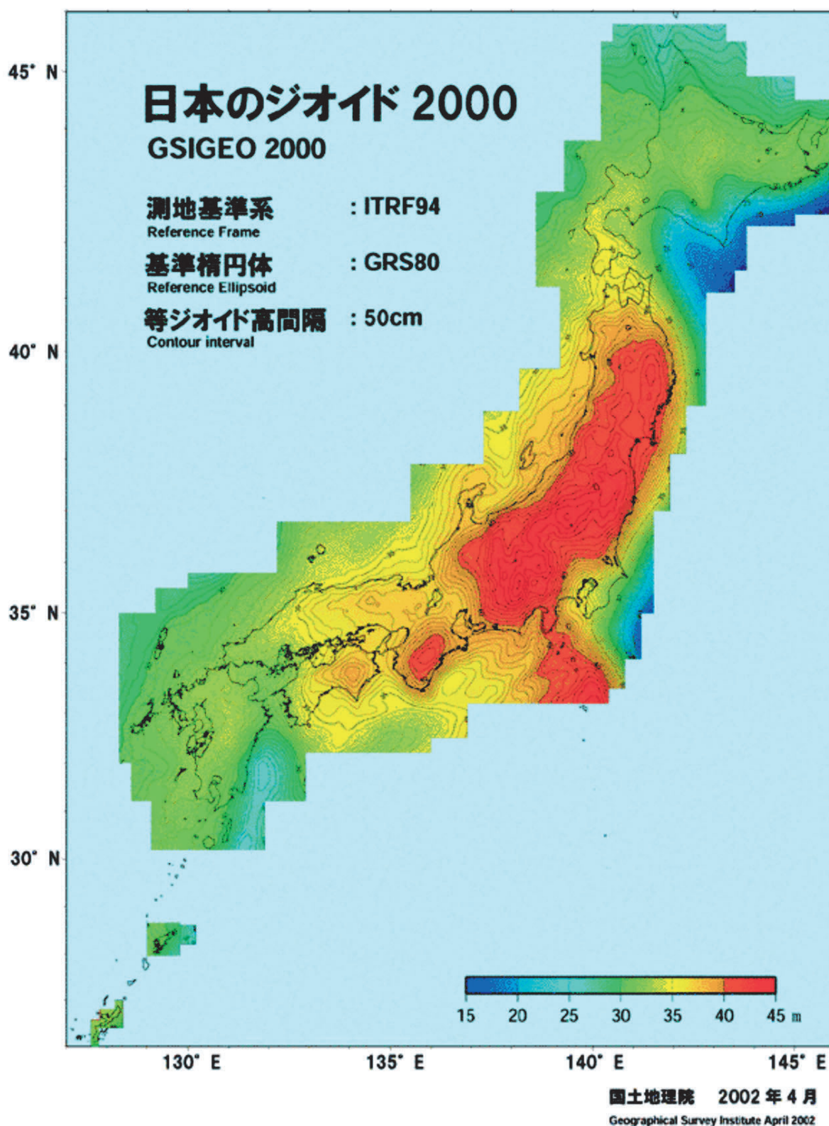
Fig. 8 Contour map of "GSIGEO2000".
