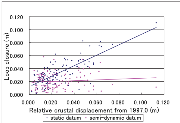
Fig. 15 Decrease of loop closure by semi-dynamic datum
