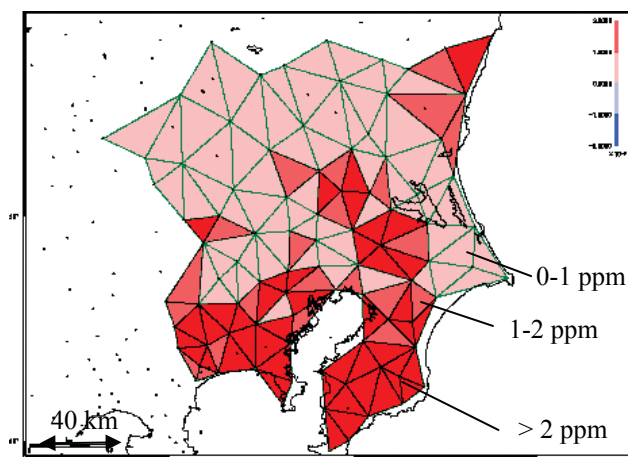
Fig. 11 The maximum shear strain accumulated in 1997–2006 due to plate subduction (Kanto district). Each color corresponds to the shown magnitude of the strain.
