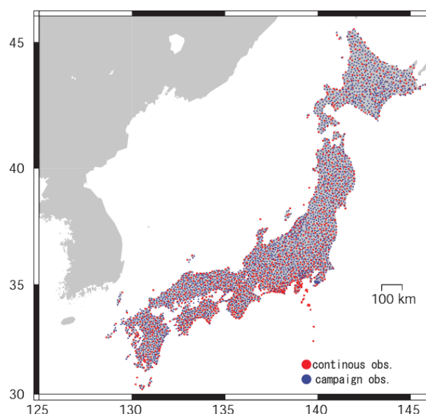
Fig. 1 Distribution of the GPS observation sites for crustal monitoring in Japan
